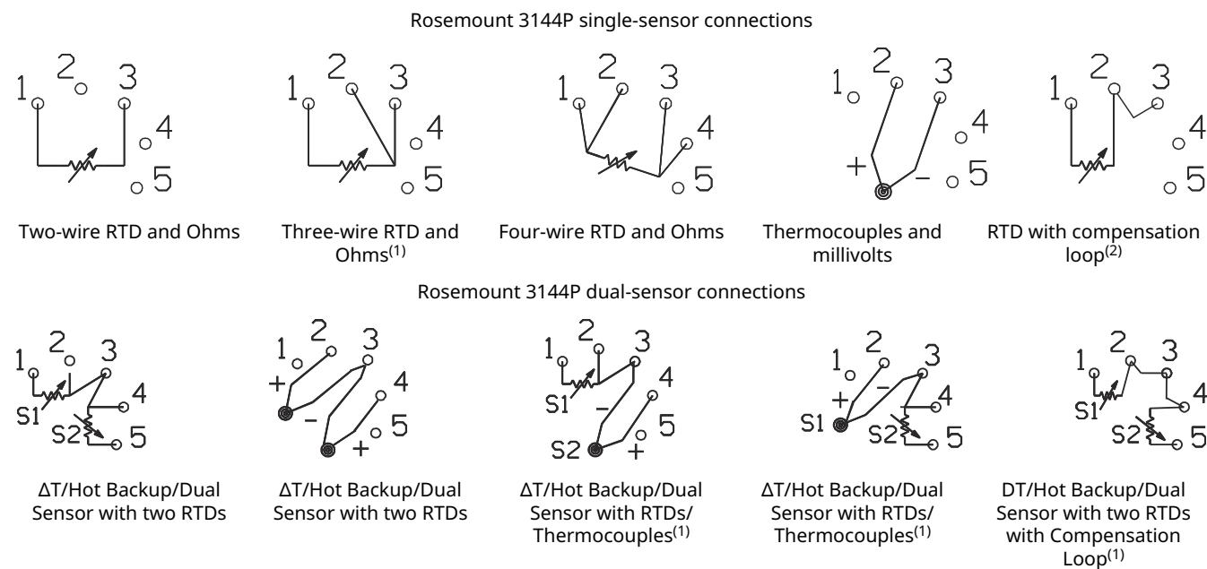
Figure 8: HART/4-20 mA
